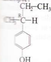
4-sec-butilfenol (A)
