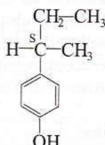
(S)-4-sec-butilfenol (B)
